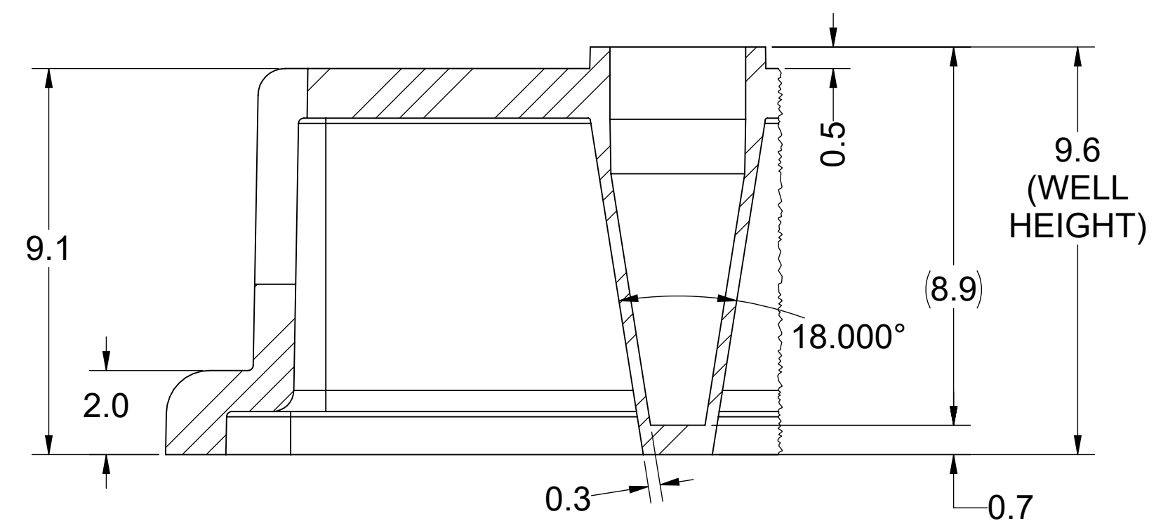
DETAIL C
