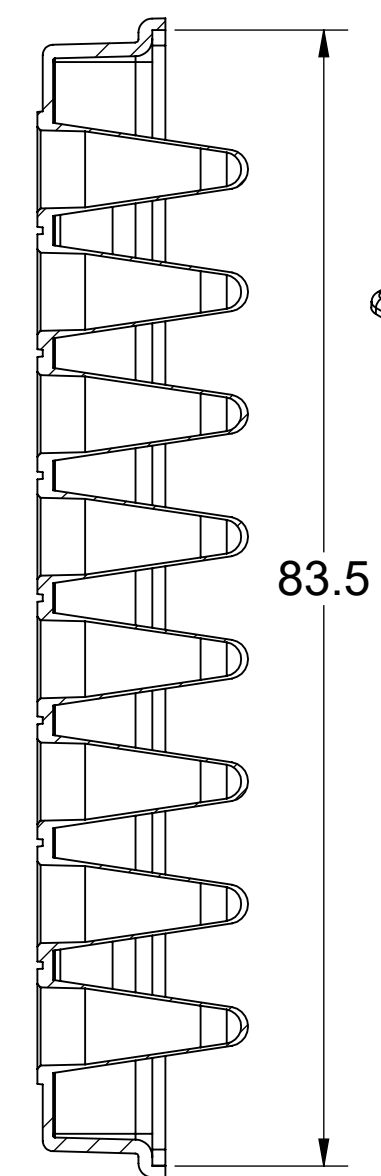
SECTION B-B
