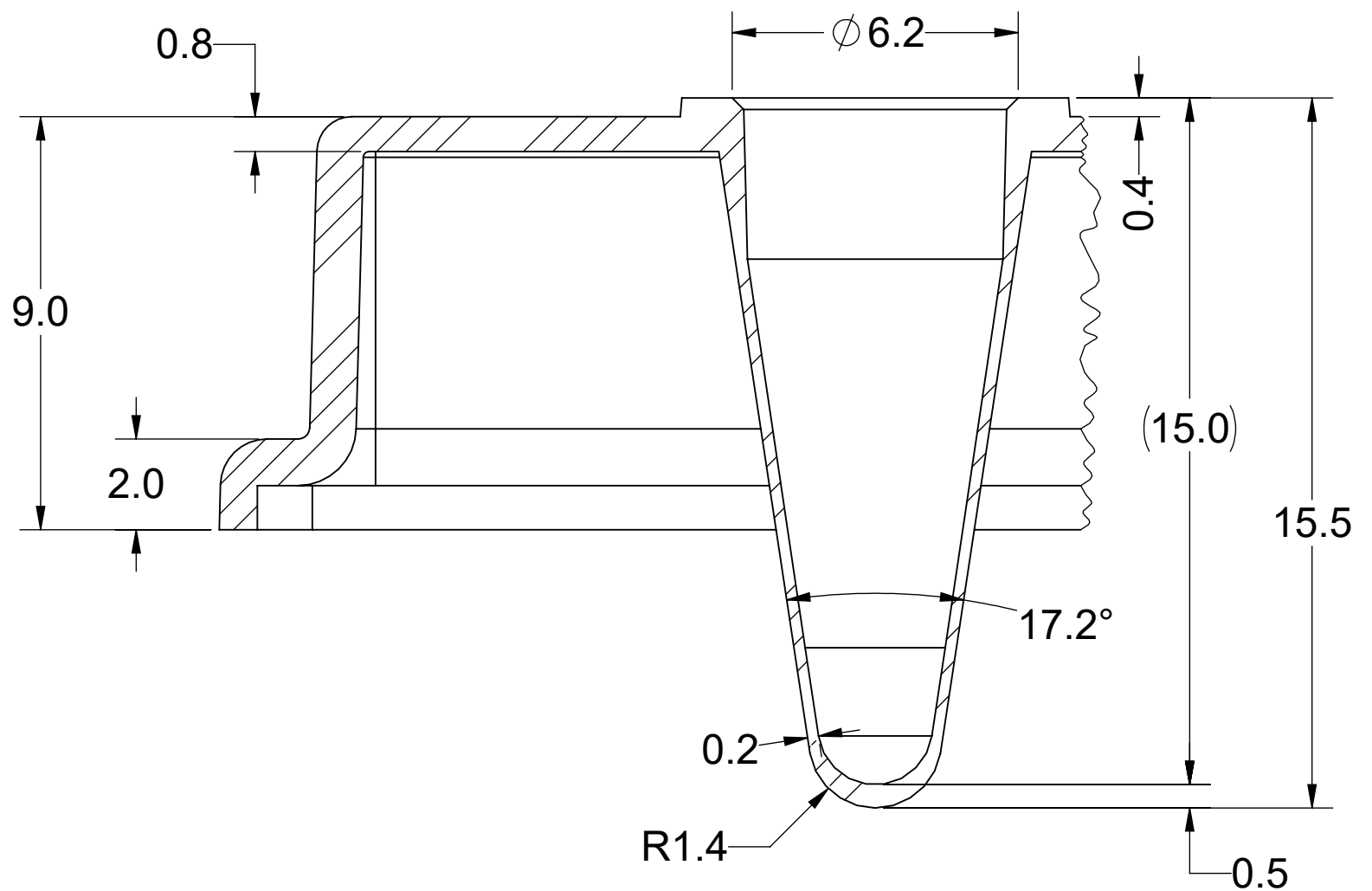
DETAIL C
