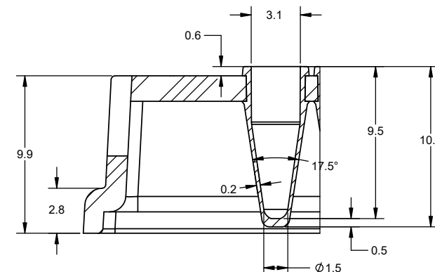
DETAIL W
