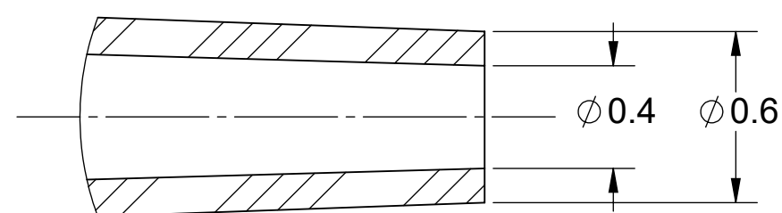
DETAIL B
