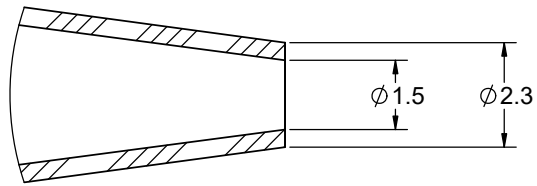
DETAIL B
