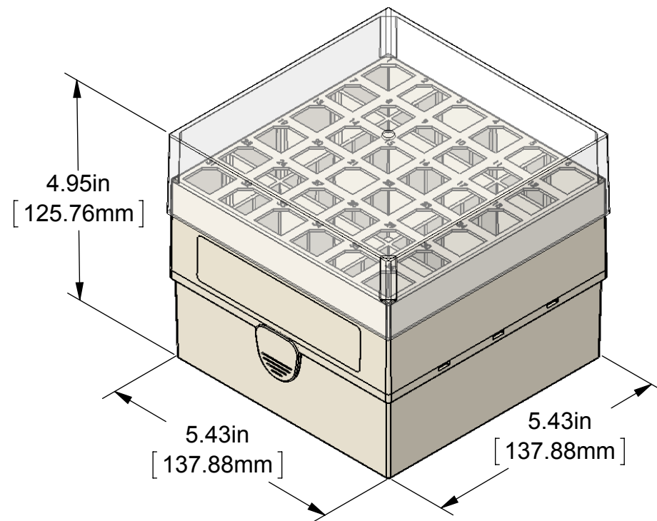
15mL TUBE RACK (CLOSED)
