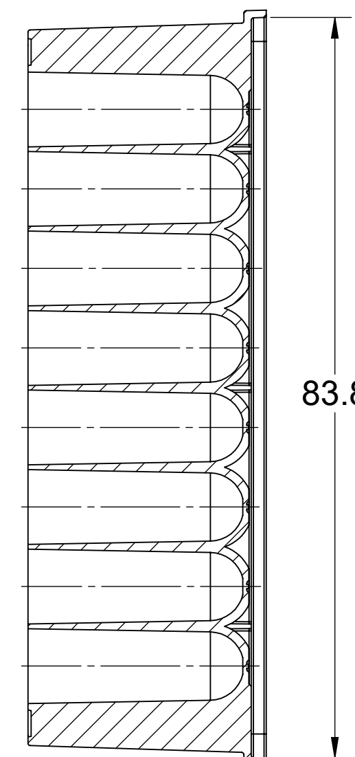
SECTION C-C
