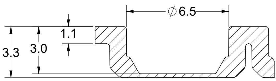
DETAIL C
