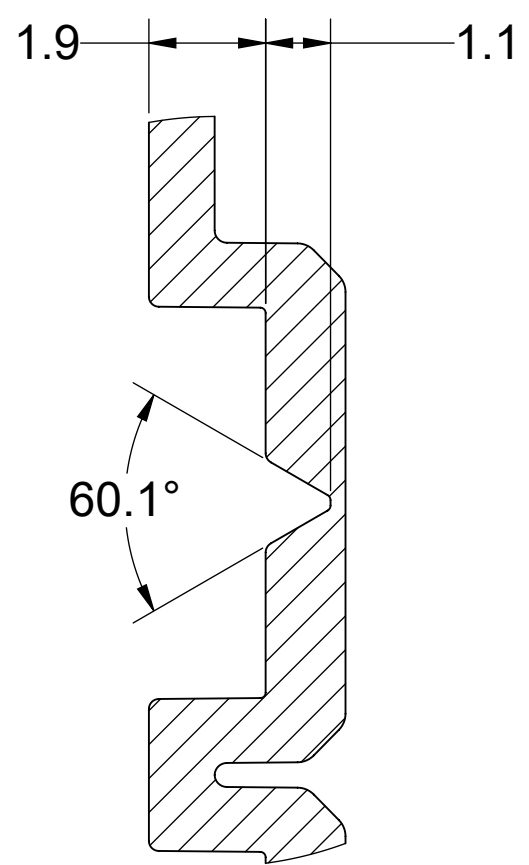
DETAIL D
