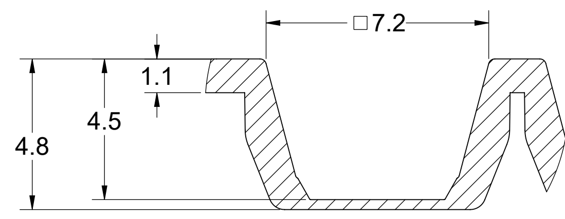
DETAIL C
