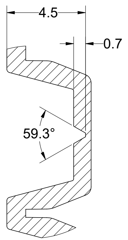
DETAIL D
