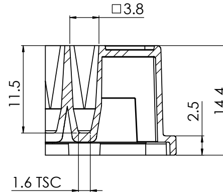
SECTION C-C SCALE 4 : 1
