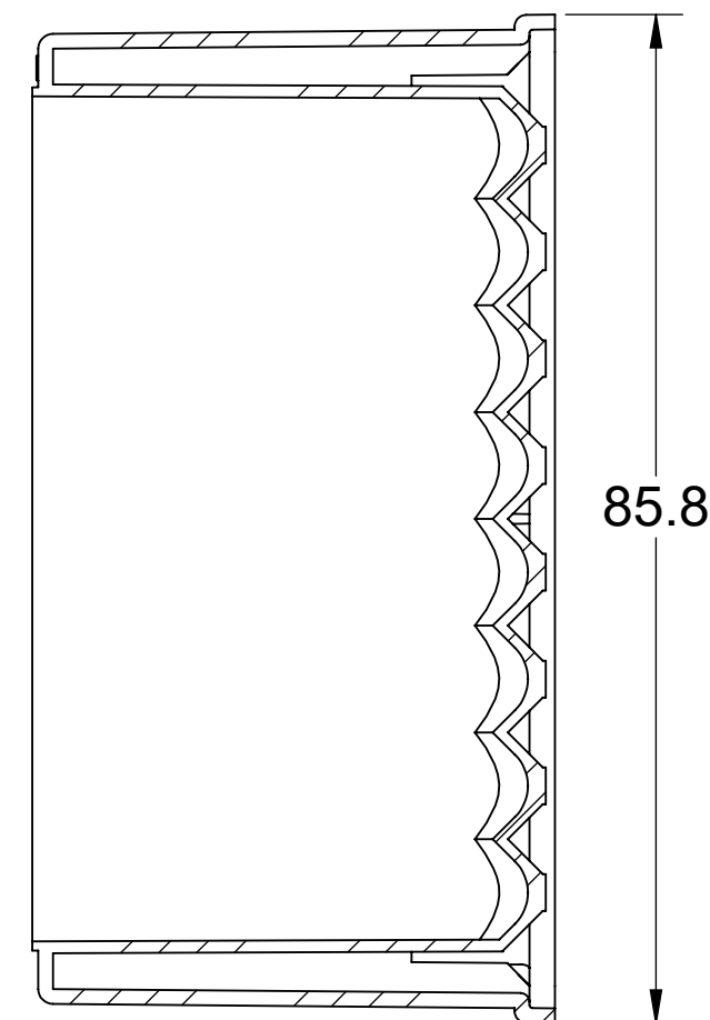
SECTION C-C
